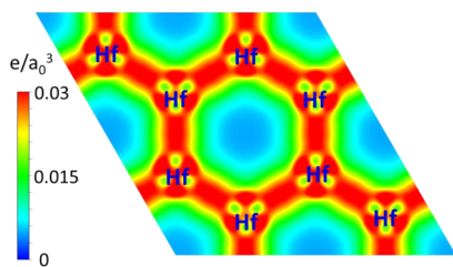
Figure 4. The 2D charge density in the Hf plane on Ir(111) substrate. Hf–Hf bonds are clearly seen and they are responsible for the observed honeycomb structure.
