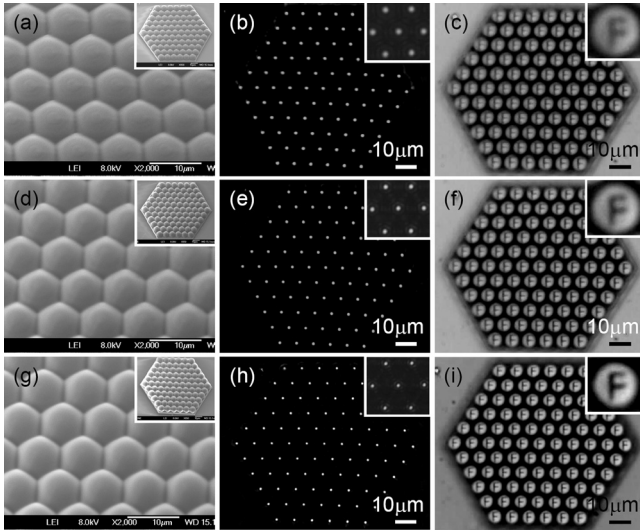
FIG. 4. High quality microlens arrays with designable NAs. (a), (d), and (g) Titled-view SEM images of gapless HMLAs with the same size and different heights. The heights of microlens are 1.2\ \mu\text{m} , 1.8\ \mu\text{m} , and 2.4\ \mu\text{m} , respectively. The insets are their whole SEM images. (b), (e), and (h) are their focal spots. (c), (f), and (i) are their arrays of miniaturized “F” images. The six insets are the locally magnified images which showed higher resolution and clearer imaging realized by these high quality HMLAs.
