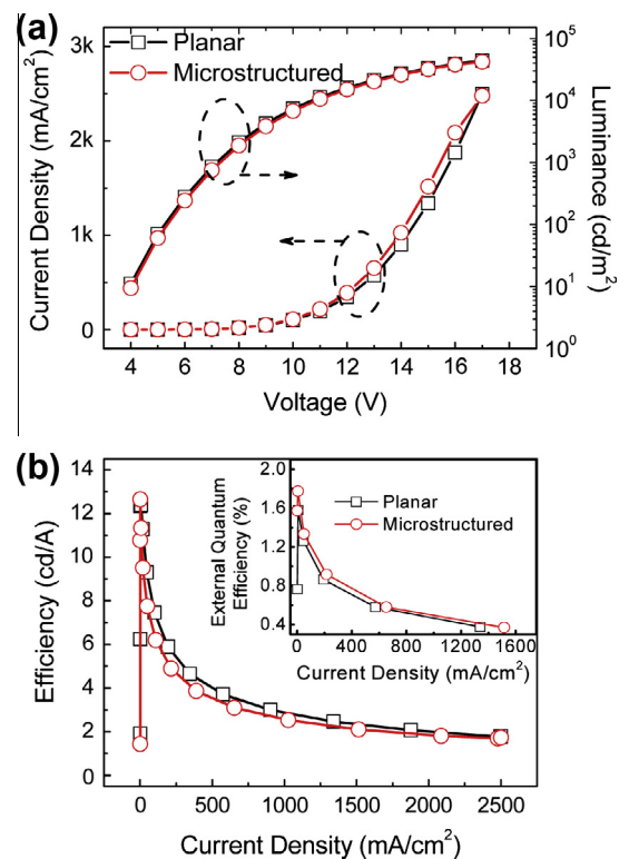
Fig. 5. (a) Current density–voltage–luminance and (b) efficiency–current density characteristics of the planar and microstructured WTOLEDs. Inset in (b): external quantum efficiency–current density characteristics of the planar and microstructured WTOLEDs.
