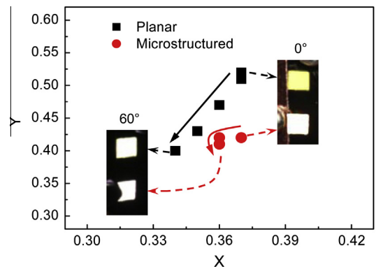
Fig. 4. CIE coordinates of the planar and microstructured WTOLEDs at different viewing angles. Inset: photograph of the operating WTOLEDs with and without the microstructure at observation angles of 0° and 60°.
