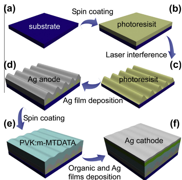
Fig. 1. Schematic fabrication process of a microstructured WTOLED. (a) Cleaning the glass substrate, (b) spin coating photoresist, (c) introducing periodic microstructure by two-beam laser interference lithography, (d) depositing Ag anode, (e) spin coating PVK: m-MTDATA and (f) depositing organic and cathode layers.
