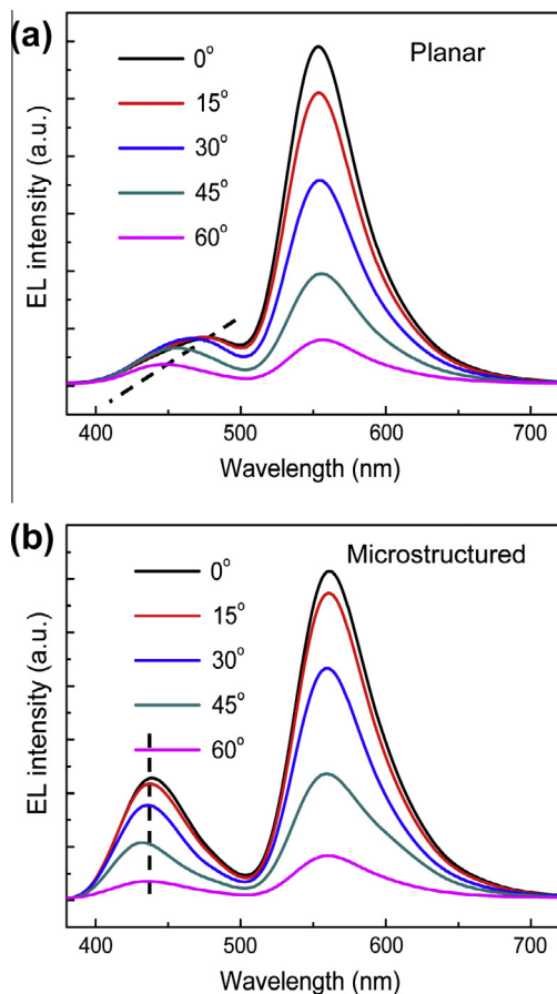
Fig. 3. EL spectra of the planar (a) and microstructured (b) WTOLEDs at viewing angles of 0°, 15°, 30°, 45°, 60° off the surface normal.
